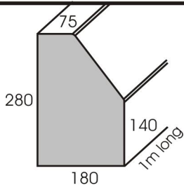
Modcon Kerbing Type 010
