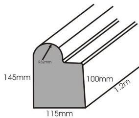
Modcon Kerbing Type 008
